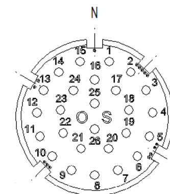
00008825 E-Part / male 26 pins
