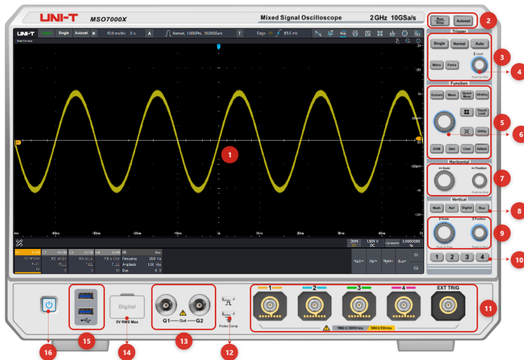
Figure 3 Front Panel
