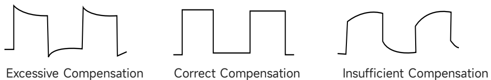
Figure 2 Compensating Calibration of Probe
