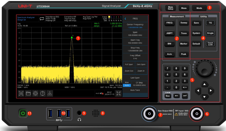
Figure 1-1 Front Panel
