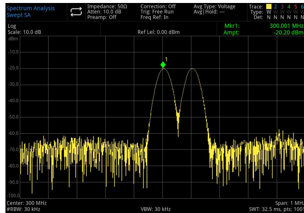
Figure 3-6 Distinguished Two Equal-Amplitude Signal (1)
