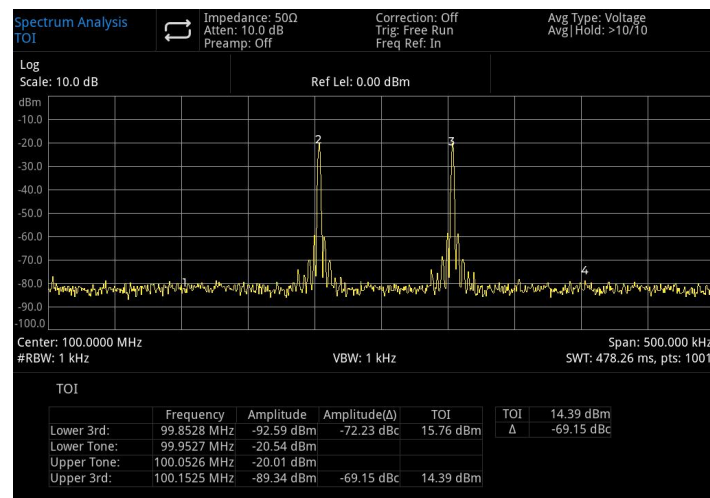
Figure 5-4 TOI
