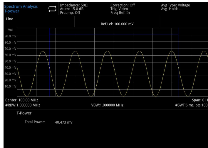
Figure 5-2 Time Domain Power
