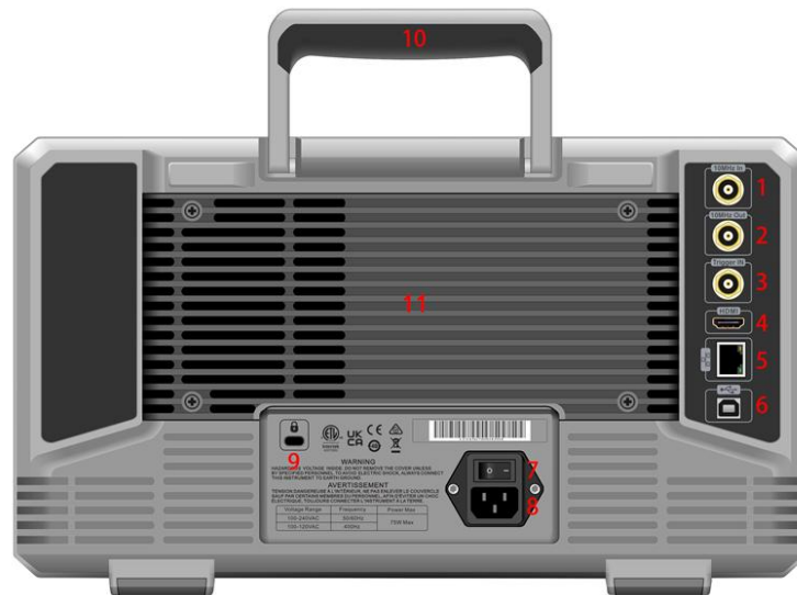
Figure 1-3 Rear Panel
