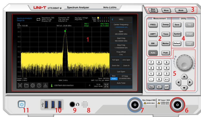
Figure 1-1 Front Panel
