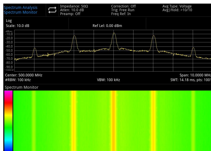
Figure 5-6 Spectrum Monitoring
