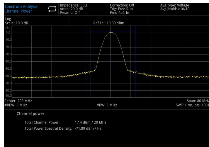
Figure 5-1 Channel Power
