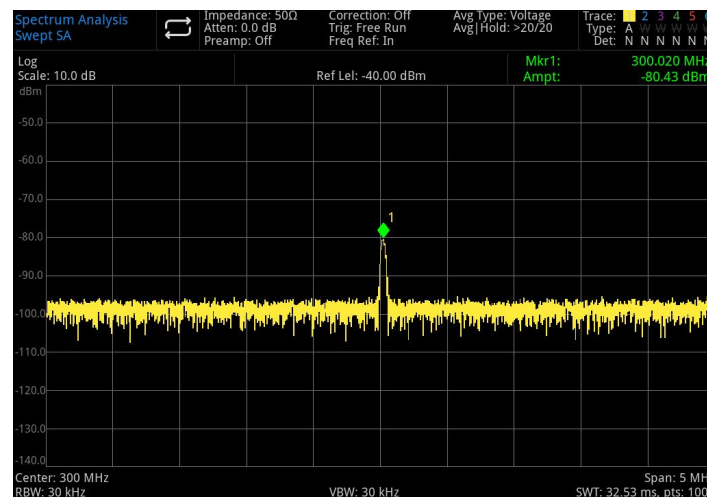
Figure 3-14 Trace Averaging
