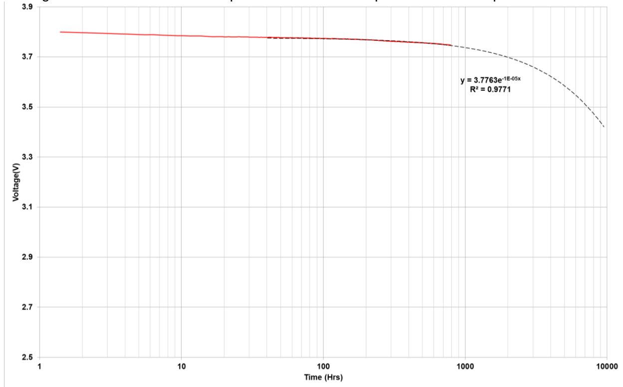
Figure 7, typical self-discharge on LY13R816025M227R-L, after 2 hours of charge
