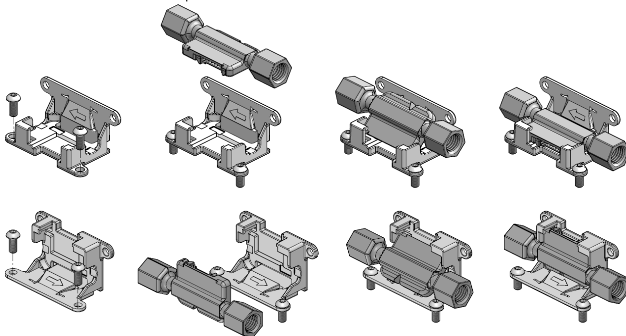
Figure 5: Mounting guidelines for the SLF3S-1300F sensor into the SLF3x mounting clamp
