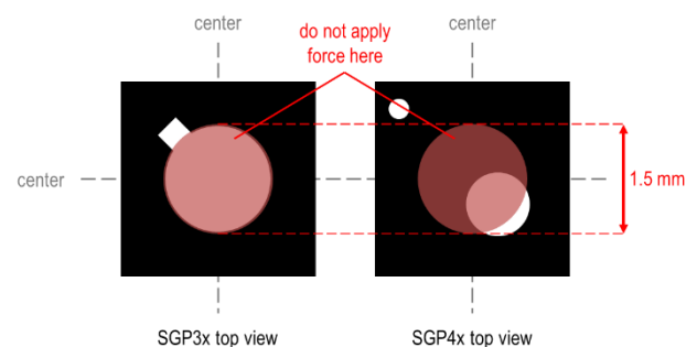
Figure 2 Areas of the sensor suitable for application of force during mounting process. Force must only be applied outside the red area.
