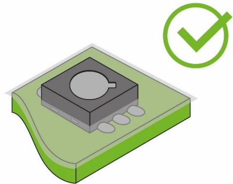
Figure 7 If conformal coating is applied, the top surface of the sensor must remain free of coating.
