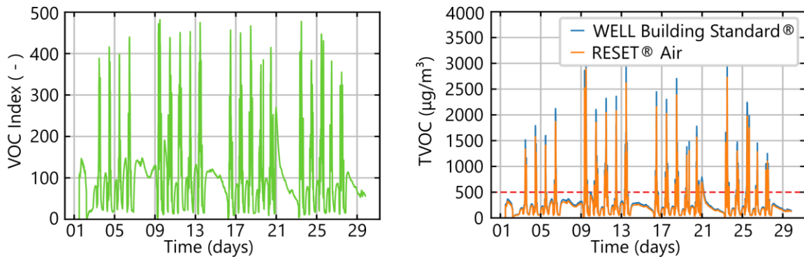
Figure 6. VOC Index (left) and corresponding \text{TVOC}_{\text{Isobutylene}} and \text{TVOC}_{\text{Mølhave}} concentration outputs according to RESET® Air and WELL Building Standard®, respectively (right).
