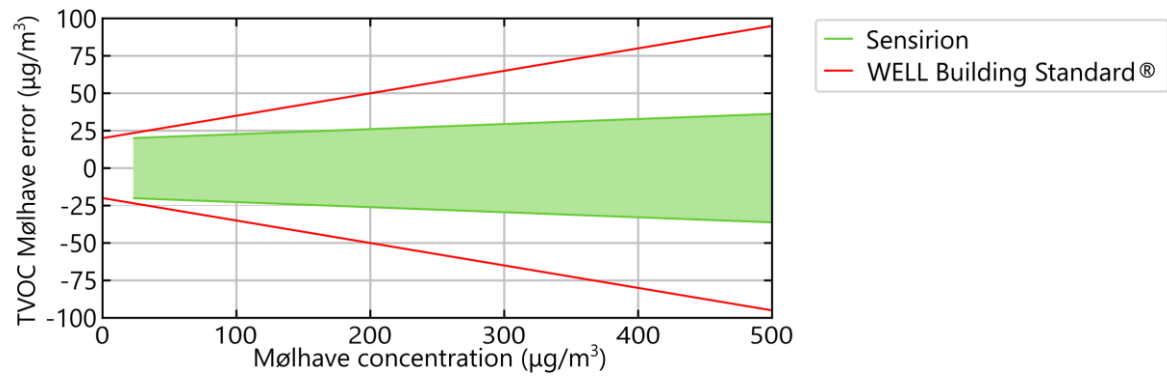
Figure 8. Accuracy of Sensirion’s sensors, as a function of TVOC Mølhave concentration (green). The error is within the maximum allowed error according to the WELL Building Standard ( \pm 20 \mu\text{g}/\text{m}^3 + 15\% measured value).
