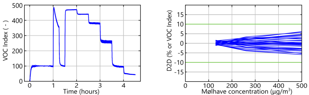
Figure 7. Repeated measurement of 30 sensors under the laboratory conditions presented in Section 2.1 (left). The corresponding device-to-device variation (D2D) is reported as a function of the Mølhave concentration.
