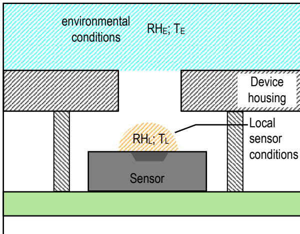
Figure 5: The sensor measures the local conditions at the sensing element ( RH_L ; T_L ). In order to achieve good measurements this local conditions need to correspond to the conditions of the environment under test (i.e. RH_E ; T_E ).
