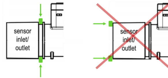
Figure 2. The O-ring (green) should be placed in the intended groove and sealing should occur through a radial force (left image).
