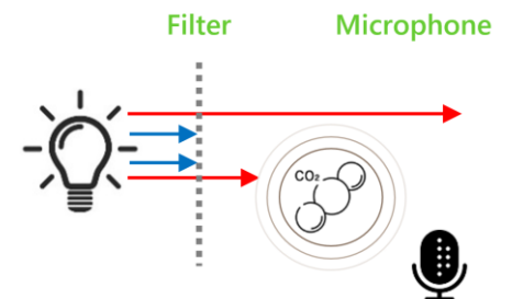
Illustration of a Photoacoustic NDIR setup
