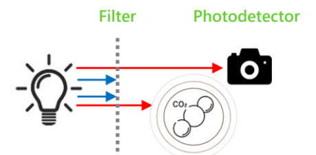
Illustration of a Transmissive NDIR setup
