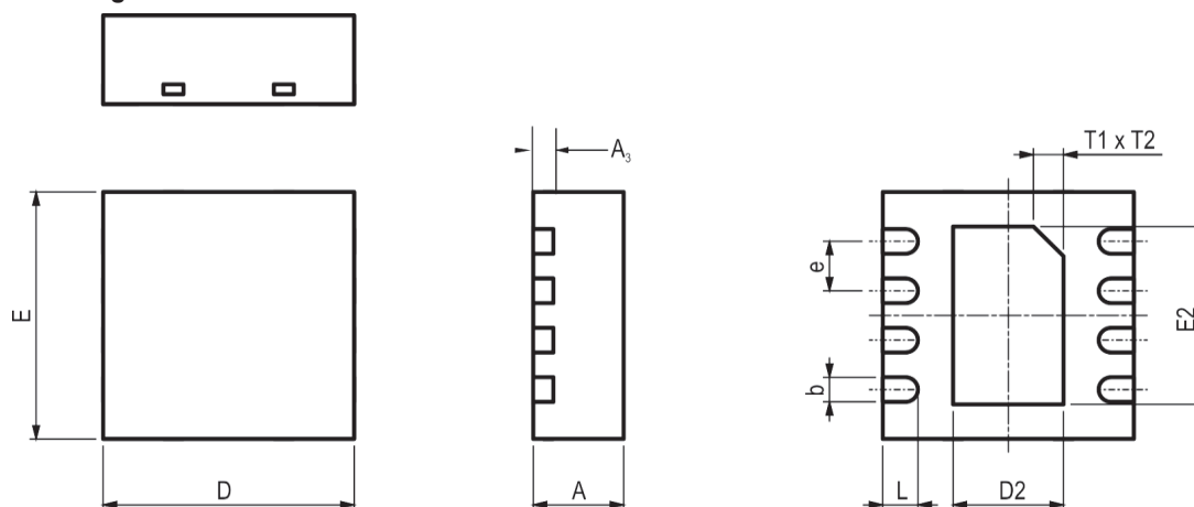
Figure 6. Dimensional drawing of STS32/33-DIS sensor package
