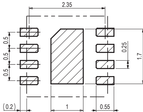
Figure 7. Recommended metal land pattern (left) and stencil apertures (right) for the STS32/33-DIS. The dashed lines represent the outer dimension of the DFN package. The PCB pads (left) and stencil apertures (right) are indicated through the shaded areas.
