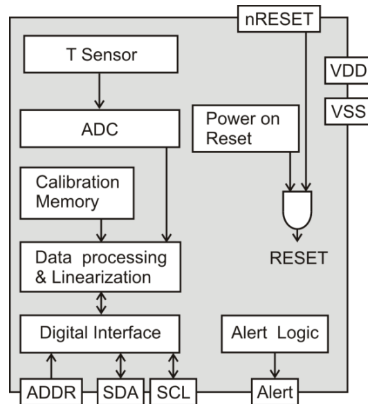
Figure 1 Functional block diagram of the STS32/33-DIS. The CMOSens™ technology allows providing for a fully calibrated I2C signal.
