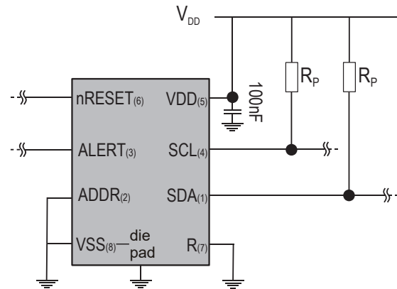
Figure 3. Typical application circuit. Please note that the positioning of the pins does not reflect the position on the real sensor. This is shown in Table 6.
