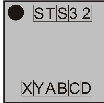
Figure 5. Top view of the STS32/33-DIS illustrating the laser marking.
