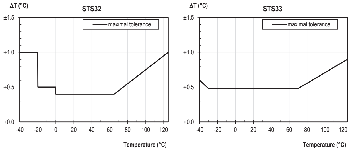
Figure 2. Temperature accuracy of the STS32 (left) and STS33 (right), respectively.
