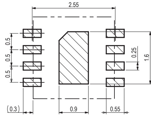
Recommended Stencil Aperture
