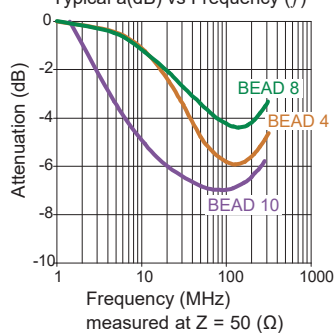
Typical a(dB) vs Frequency (f)
