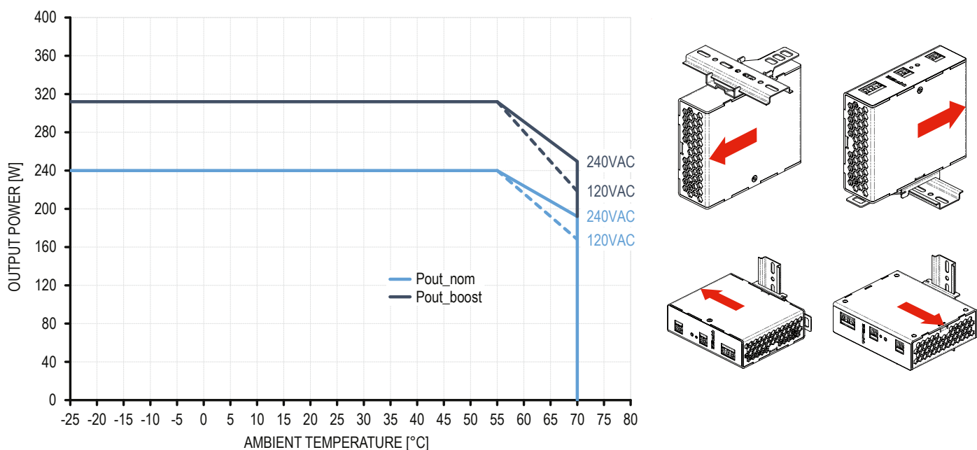
Fig. 14: Available output power in dependence of the ambient temperature for 90° rotated mounting position
