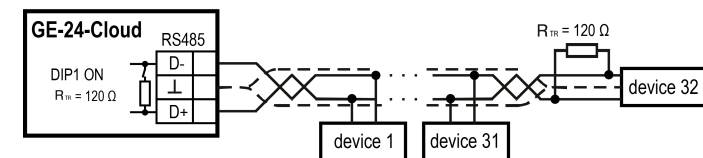
Fig. 4 Connection to RS485 interface
