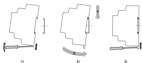
Fig. 2 – Installation
