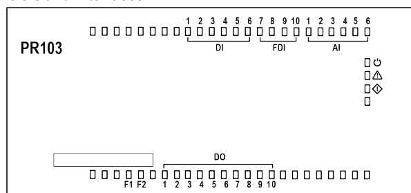
Fig. 14 – Front view
