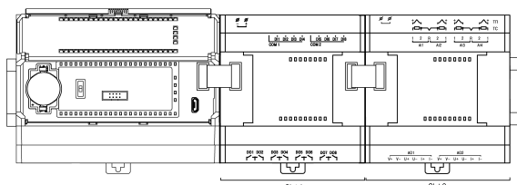
Fig. 10 – Extension modules connection
