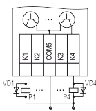
Fig. 11 – Transistor optocoupler output wiring
