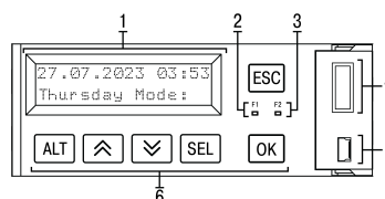
Fig. 12 – Face plate
