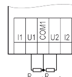
Fig. 5 – Resistance sensors wiring
