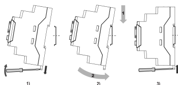
Fig. 2 – Installation
