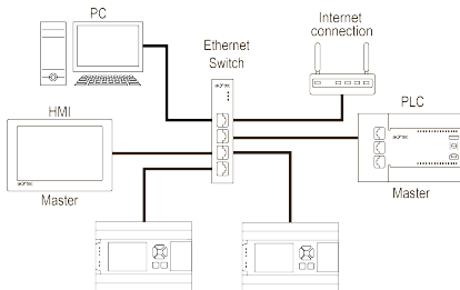
Fig. 14 – Star topology
