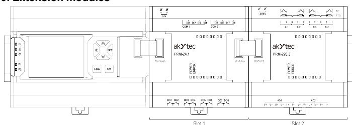
Fig. 15 – Extension modules connection
