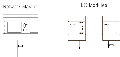
Fig. 13 – PR205 as Master
