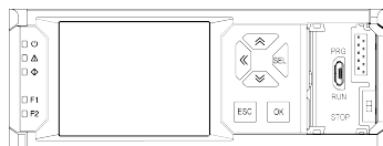
Fig. 16 – The front panel (the cover on the right is open)
