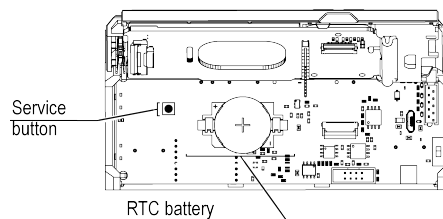
Fig. 17 – Under the front panel
