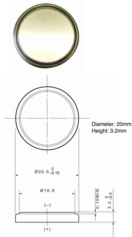
Dimension Drawing
