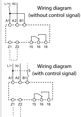
Wiring diagram (with control signal)
