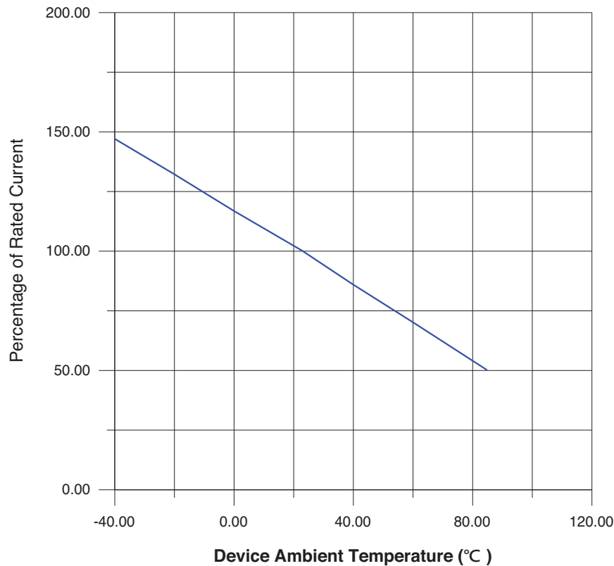
Thermal Derating Curve
