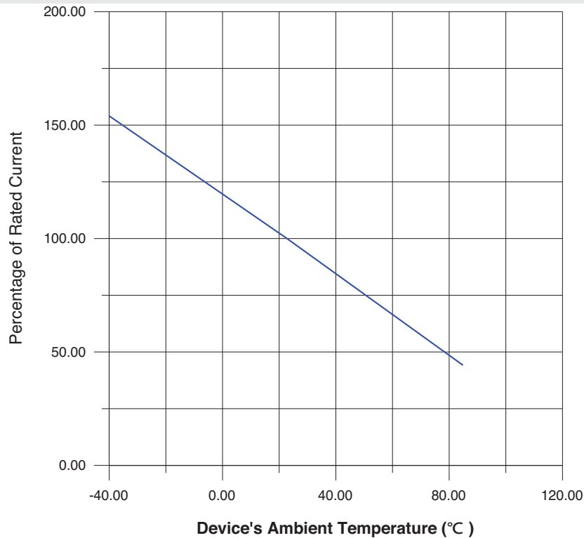
Thermal Derating Curve
