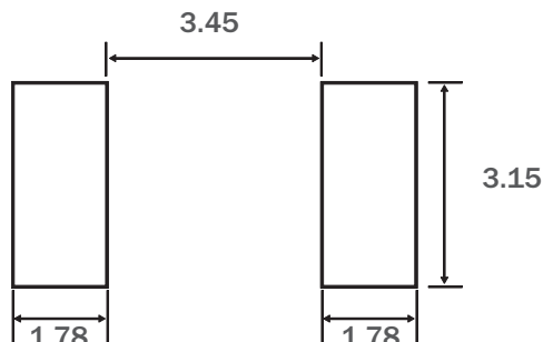
Recommended Pad Layout (mm.)
