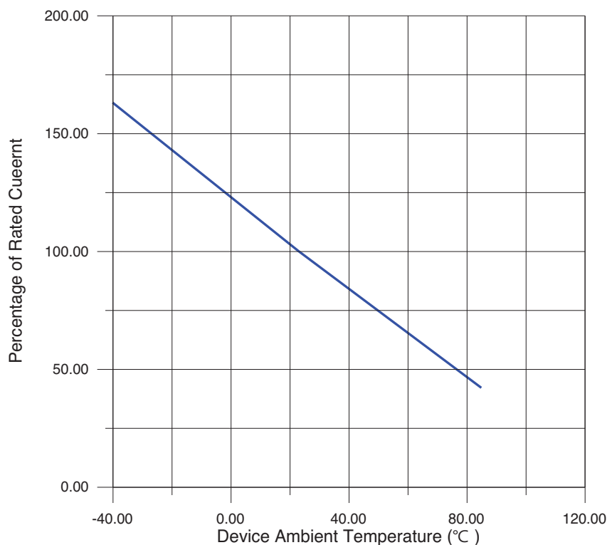
Thermal Derating Curve
