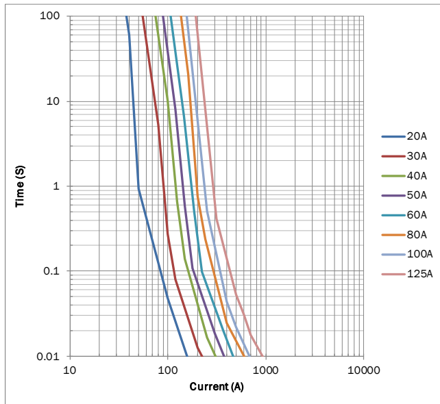
Time-Current Curve
