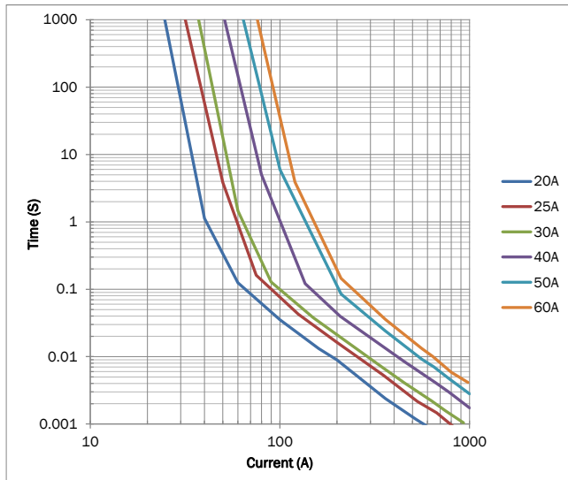
Time-Current Curve
