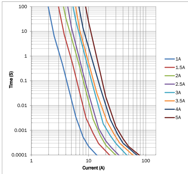
Time-Current Curve
