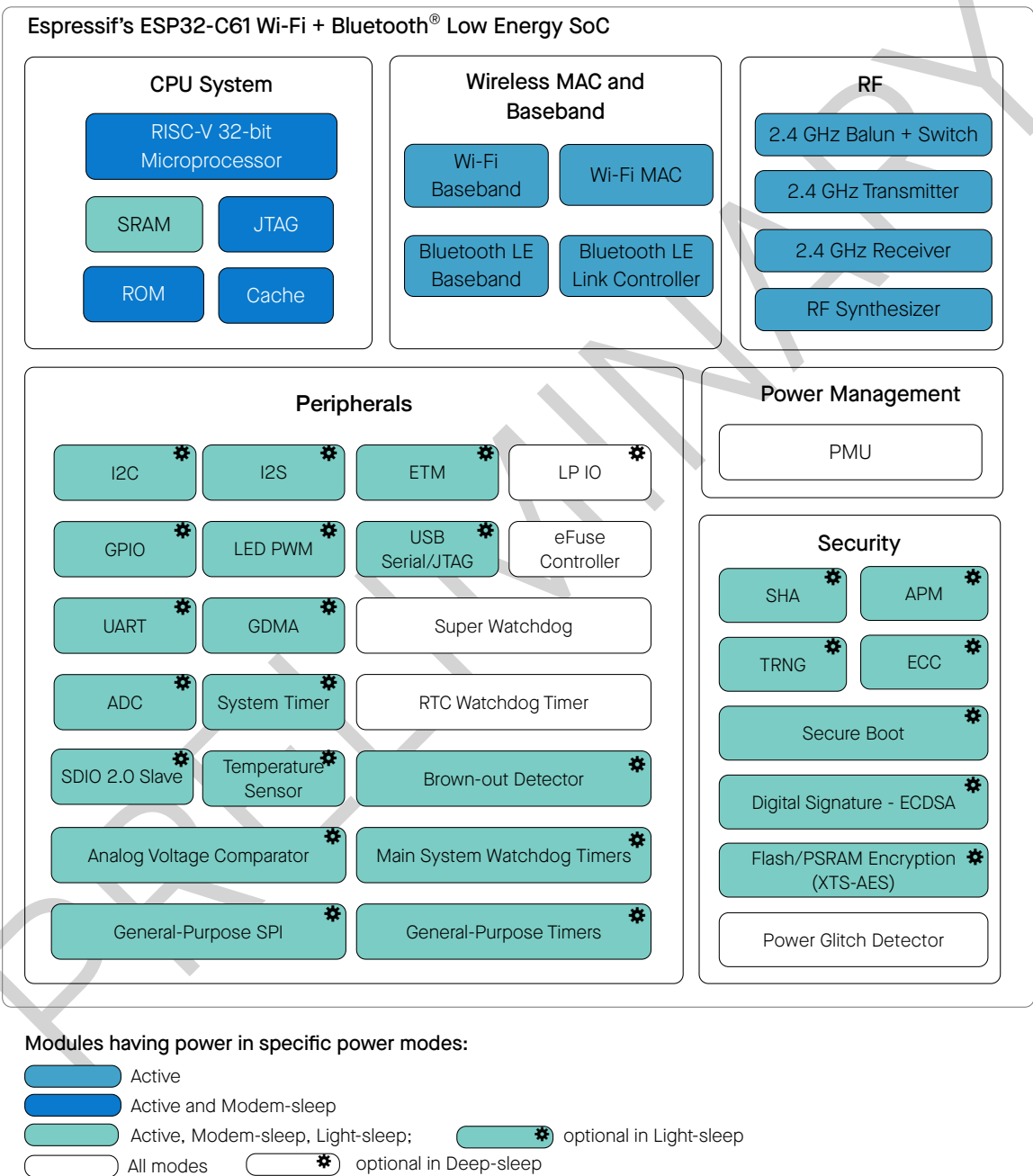
ESP32-C61 Functional Block Diagram
