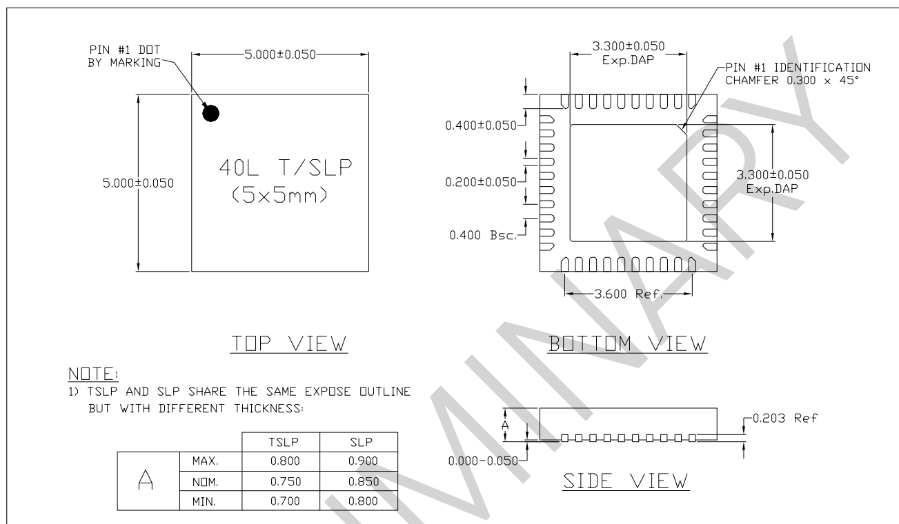
Figure 7-1. QFN40 (5×5 mm) Package
