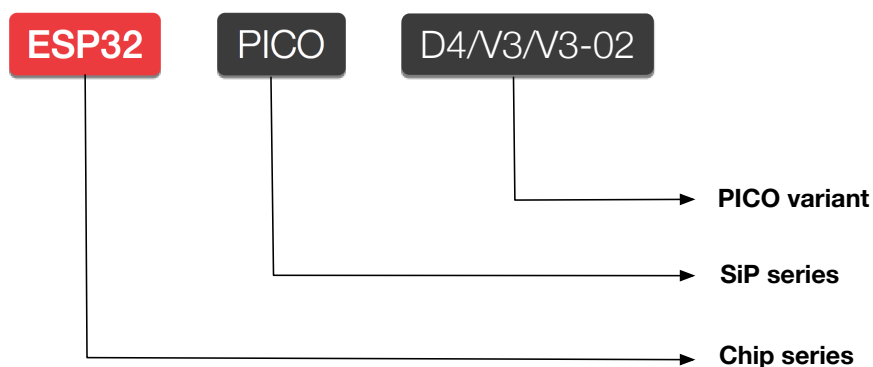
Figure 2: ESP32-PICO Series Nomenclature
