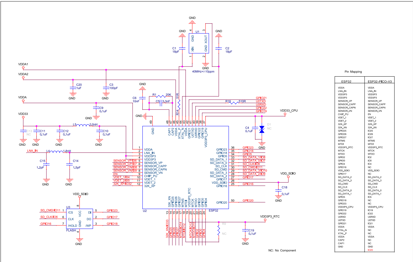
Figure 8: ESP32-PICO-V3 Schematics
