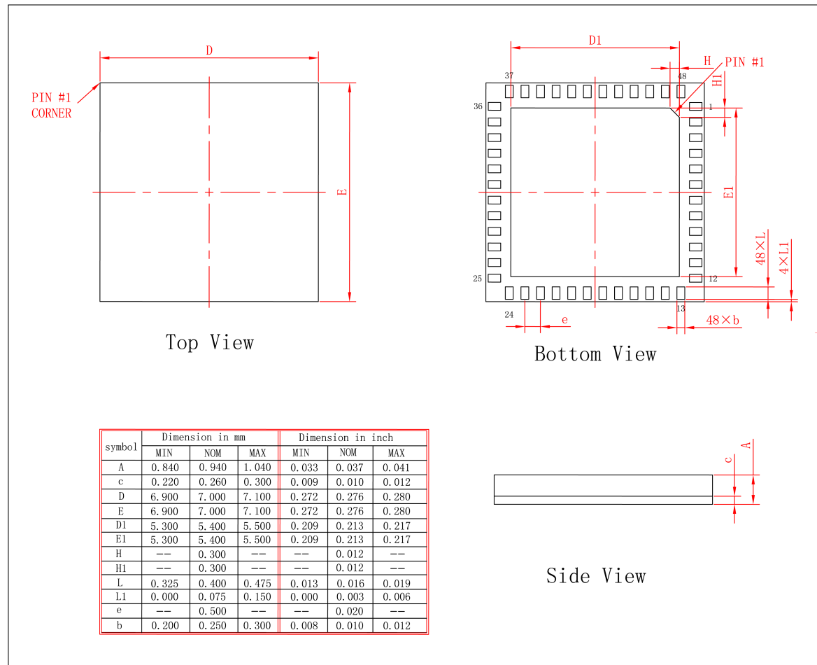
Figure 13: ESP32-PICO-D4 Package
