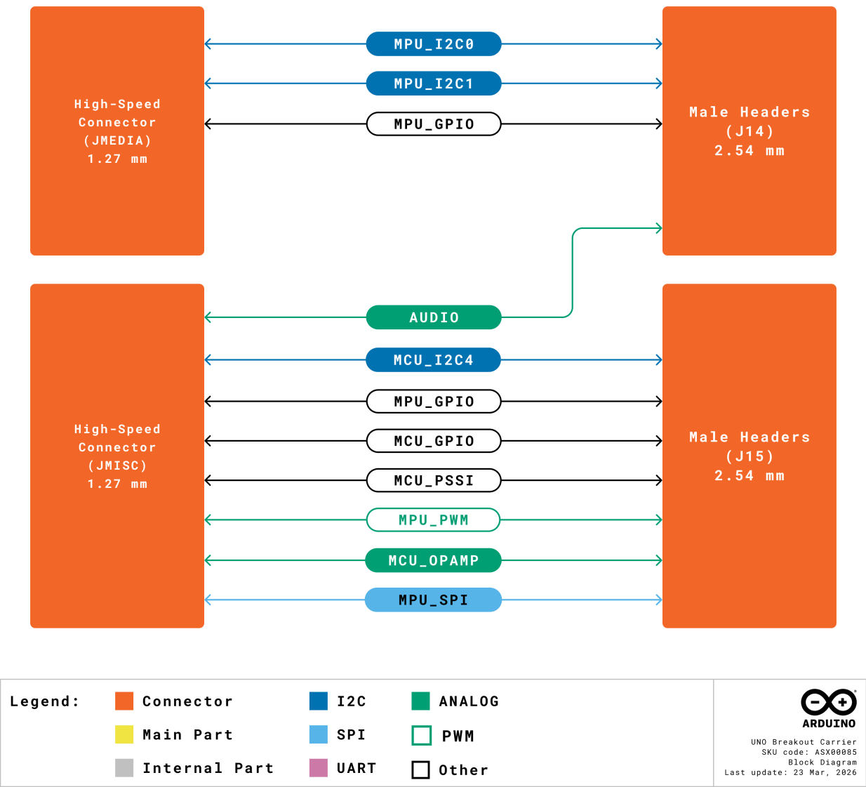
UNO Breakout Carrier Block Diagram
