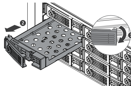
3.5-inch HDD
