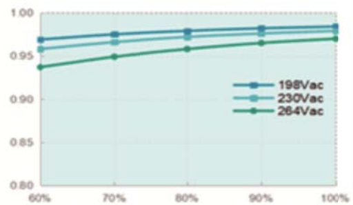
Fig.6 Efficiency-Load curve
