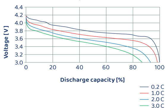
Discharge at different C-rates 1054B Rate discharge profile
