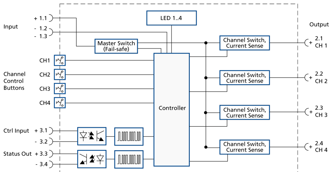
Fig. 12-1: Functional diagram
