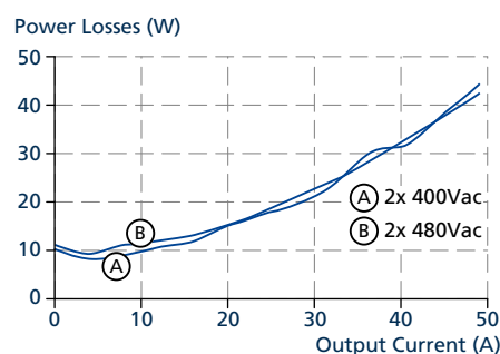
Fig. 29-4: Power Losses vs. output current at 24 V
