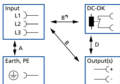
Fig. 24-1: Dielectric strength
