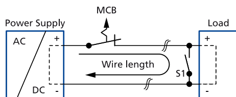
Fig. 29-5: Test circuit
