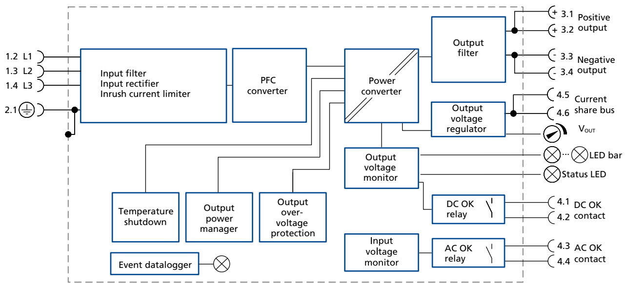
Fig. 16-1: Functional Diagram TP960.241
