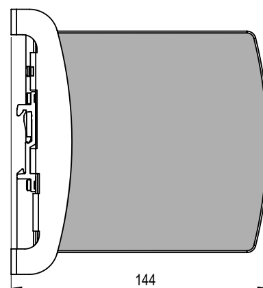
Fig. 28-6: Wall / panel mounting, side view
