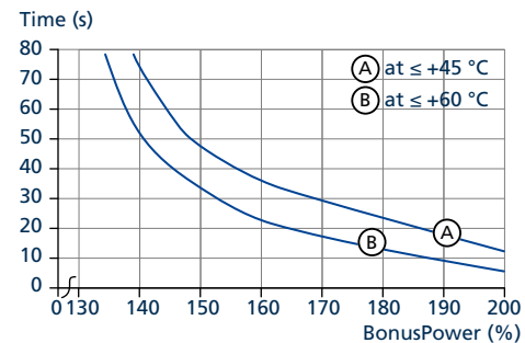
Fig. 7-4: Calculated time availability of BonusPower
