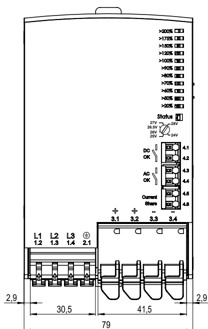
Fig. 27-1: Front view
