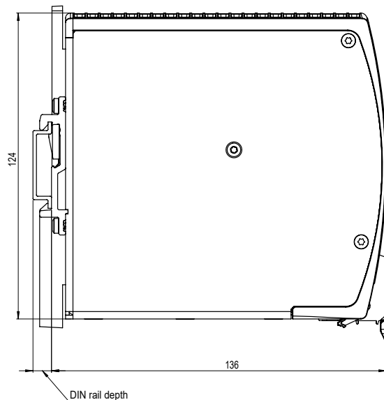
Fig. 27-2: Side view
