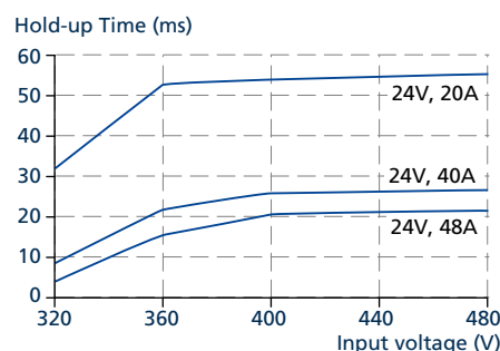
Fig. 29-2: Hold-up time vs. input voltage
