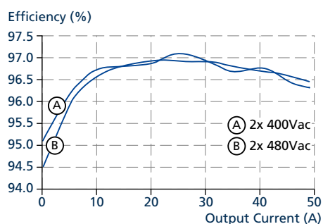
Fig. 29-3: Efficiency vs. output current at 24 V
