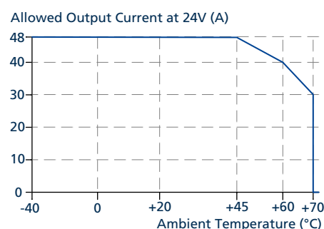
Fig. 21-1: Output current vs. ambient temp.
