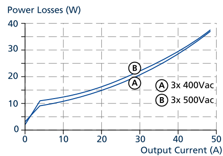
Fig. 13-2: Losses vs. output current at 24 V, typ.
