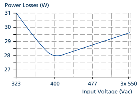
Fig. 13-4: Losses vs. input voltage at 24 V, 40 A, typ.
