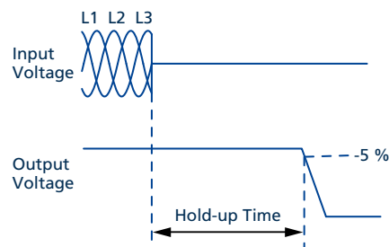
Fig. 8-2: Shut-down behaviour
