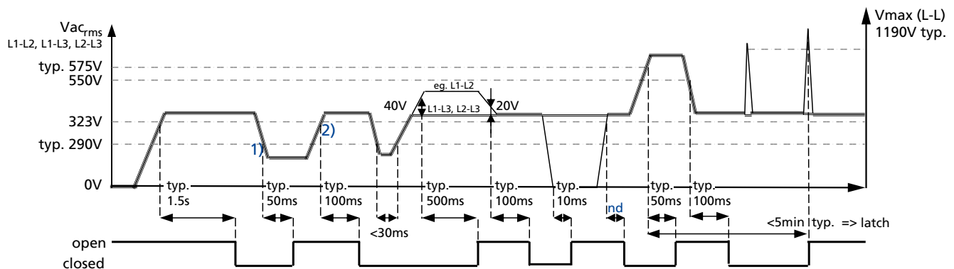
Fig. 10-1: AC OK relay contact behavior
