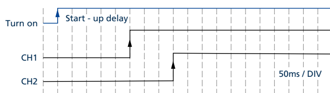
Fig. 6-1: Sequential start of the outputs
