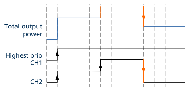
Fig. 6-2: Tripping of the channel with the lowest priority when the power budget is exceeded
