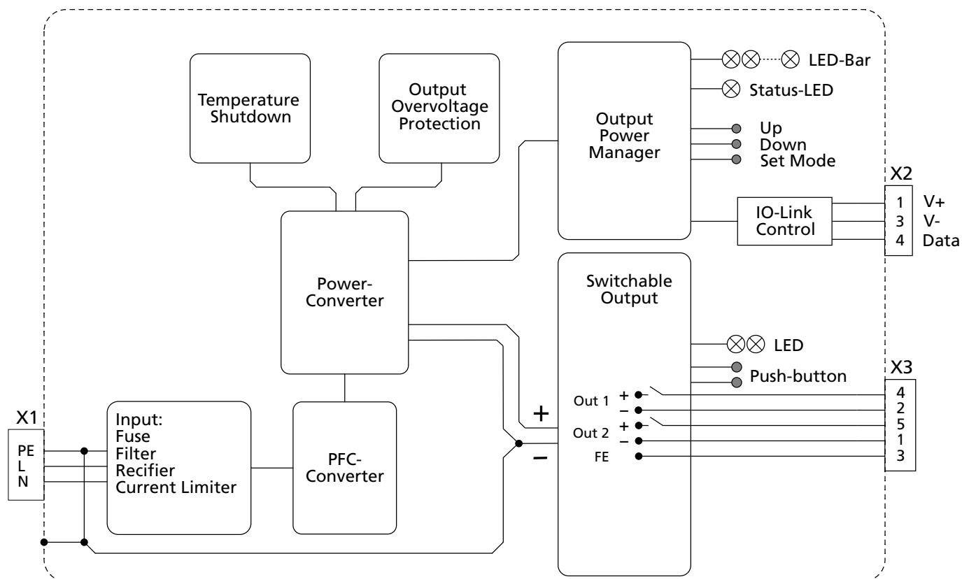
Fig. 12-1: Functional Diagram FPS300.245-016-101
