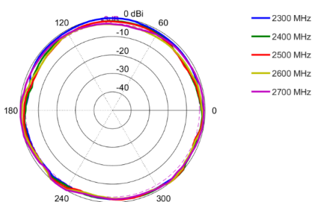
Azimuth: 2300 – 2700 MHz
