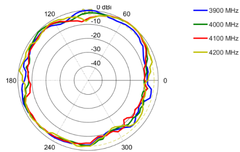
Elevation: 3900 – 4200 MHz
