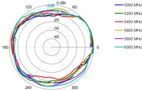
Azimuth: 5000 – 6000 MHz
