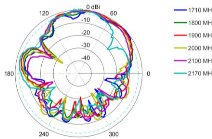
Elevation 2: 1710 – 2170 MHz
