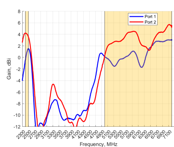
GAIN (Excluding Cable Loss): Wi-Fi Antenna
