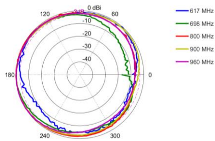
Elevation 2: 617 – 968 MHz
