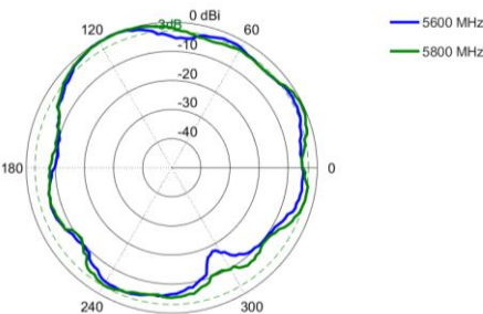
Elevation 2: 5600 – 5800 MHz
