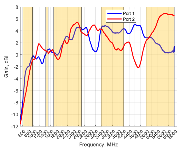
GAIN (Excluding Cable Loss): Cellular Antenna
