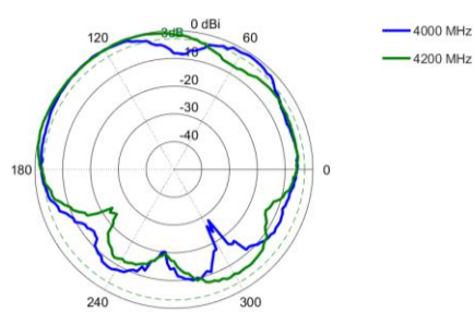
Elevation 2: 4000 – 4200 MHz
