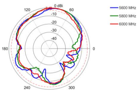
Elevation 2: 5600 – 6000 MHz
