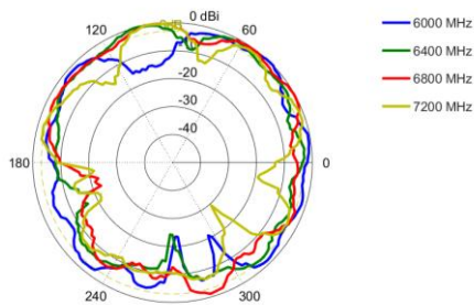
Azimuth: 6000 – 7200 MHz
