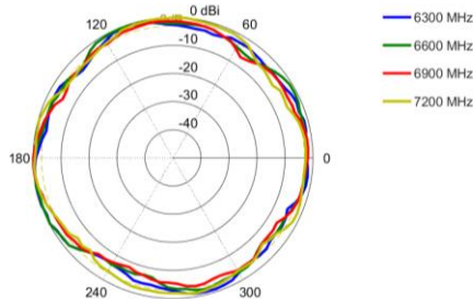
Azimuth: 6300 – 7200 MHz
