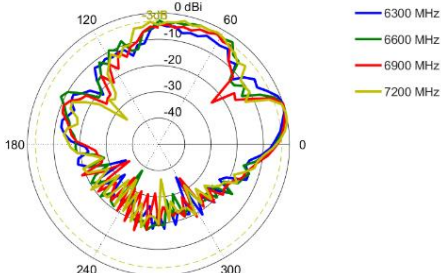
Elevation: 6300 – 7200 MHz
