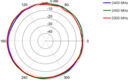
Azimuth: 2400 – 2500 MHz
