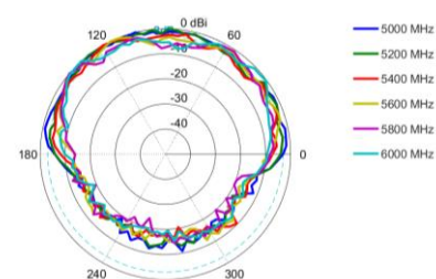
Elevation: 5000 – 6000 MHz
