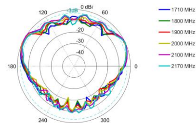
Elevation: 1710 – 2170 MHz
