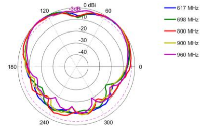
Elevation: 617 – 960 MHz
