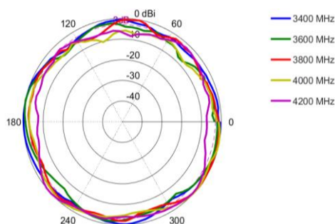
Azimuth: 3400 – 4200 MHz
