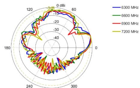
Elevation: 6300 – 7200 MHz
