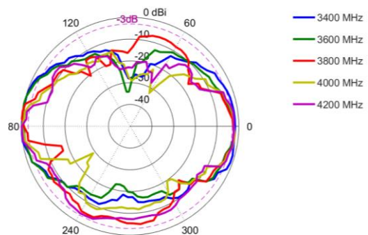
Elevation: 3400 – 4200 MHz
