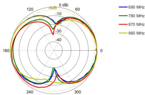
Elevation: 690 - 960 MHz
