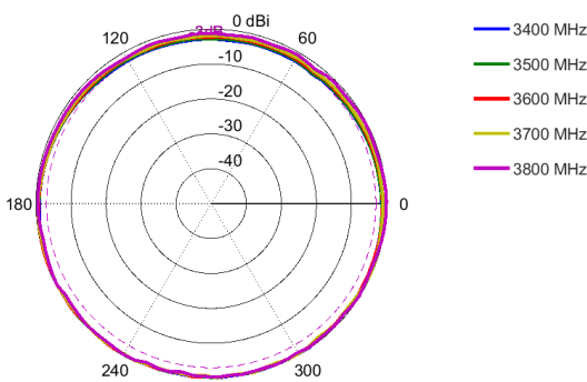
Azimuth: 3400 - 3800 MHz
