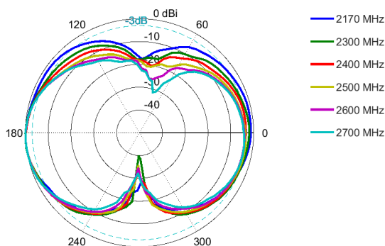
Elevation: 2170 - 2700 MHz
