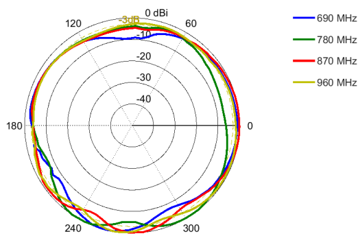
Azimuth: 690 - 960 MHz
