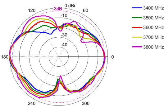
Elevation: 3400 - 3800 MHz
