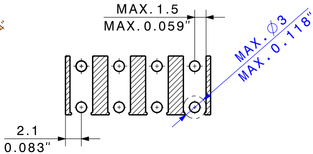
PASTE-FREE AREA
