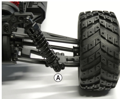
Figure 8: Rear axle
