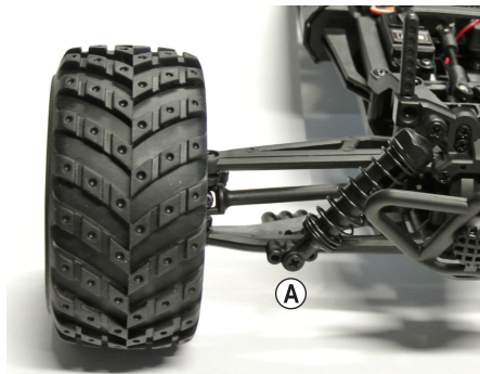
Figure 7: Front axle
