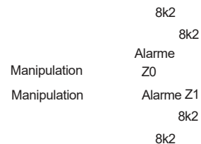
Figure 7 - Types de câblage
