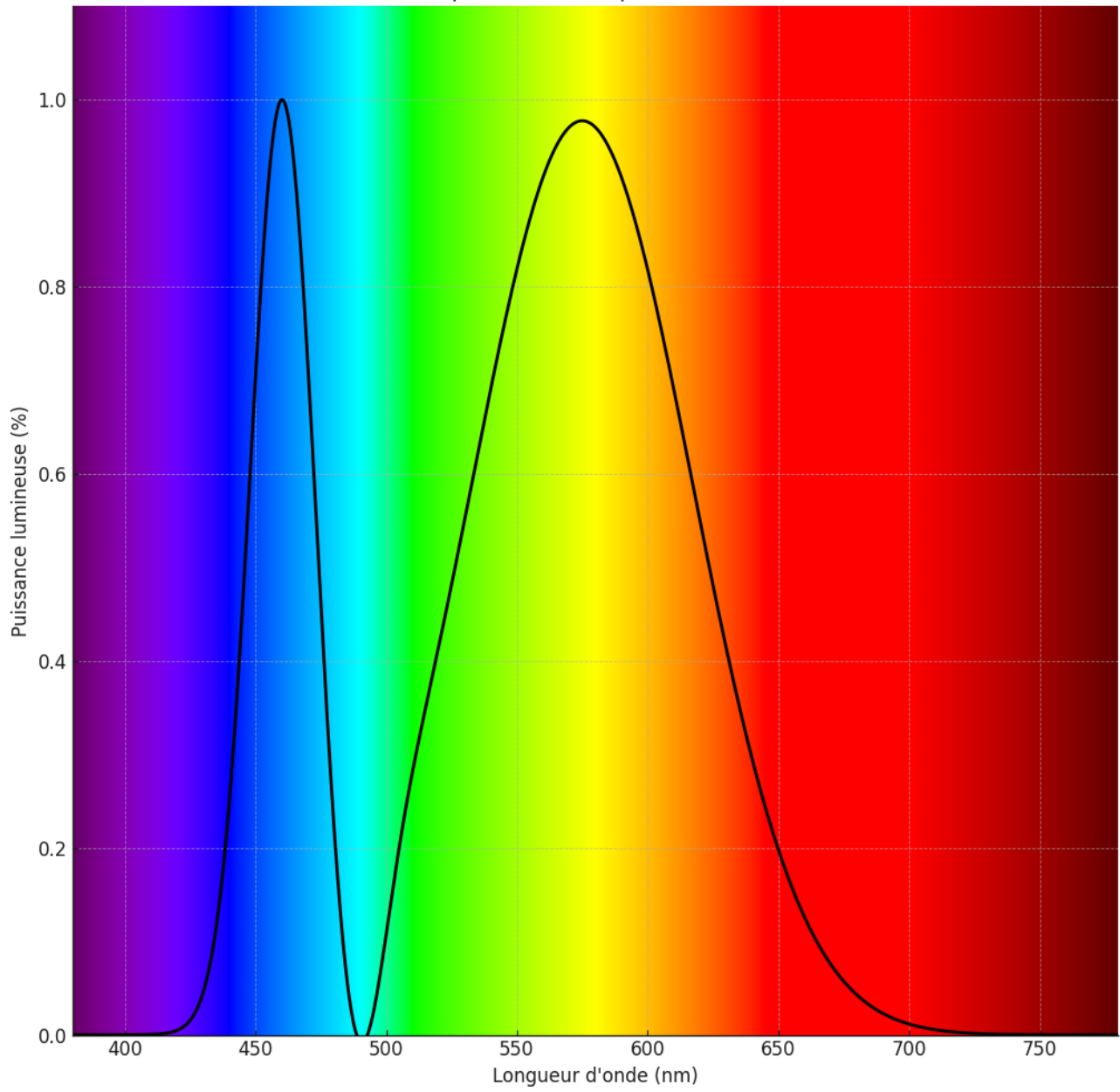
Distribution spectrale - Ampoule LED 4200K RA80
